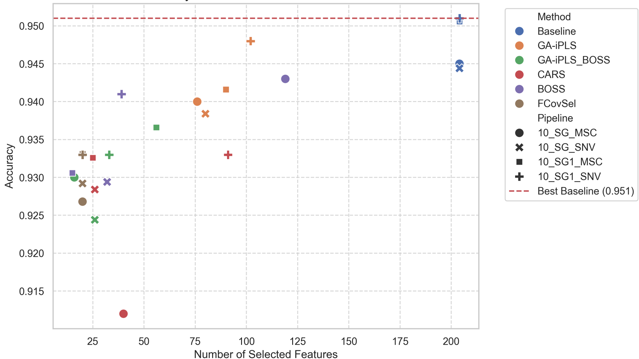
Accuracy vs. Number of Features - Salinas
